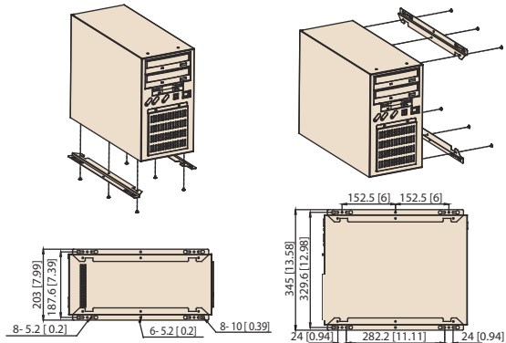
Bidirectional mounting
